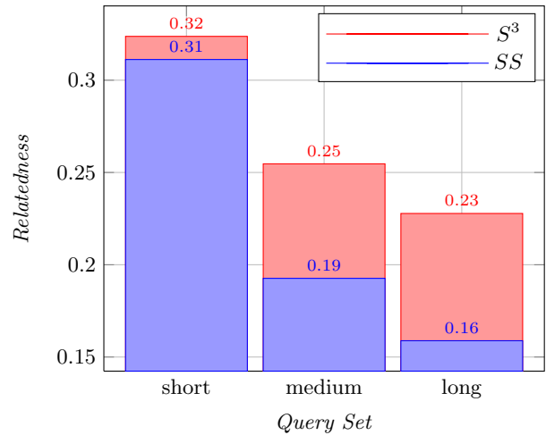
Figure 1: Per-set average relatedness computed between the list of suggestions and the given query.
